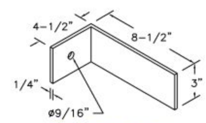
BRACKET DETAIL
