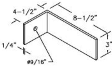
BRACKET DETAIL
