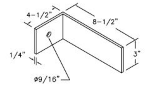
BRACKET DETAIL
