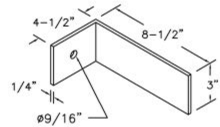
BRACKET DETAIL
