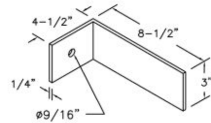
BRACKET DETAIL
