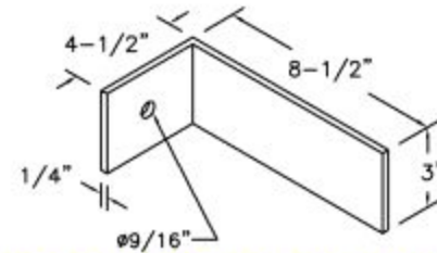
BRACKET DETAIL
